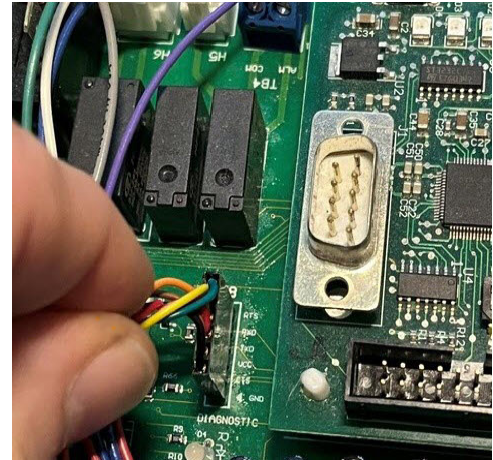
Figure 14: Diagnostic Cable Connection to Unit Controller Baseboard
